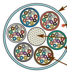
72 Fibre
