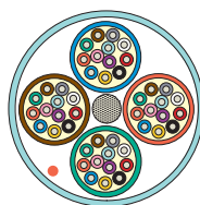
48 Fibre
